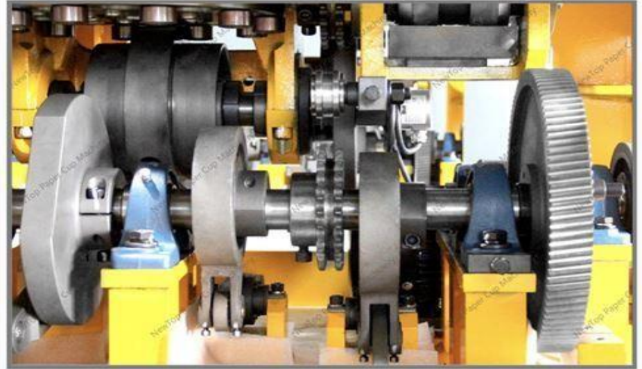
MECHANICAL TRANSMISSION
